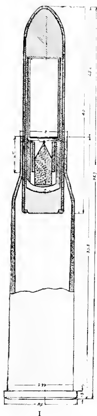
PLATE 2.—1. SKETCH OF A CARTRIDGE WITH EXPLOSIVE BULLETS; 2. CHAMBER FOR POWDER; 3. BASE OF THE CASE BEARING THE DATE 1912 AND THE AUSTRIAN EAGLE; 4. GUIDE TUBE; 5. STRIKER; 6. CHAMBERS FOR NOS. 4 AND 5.
